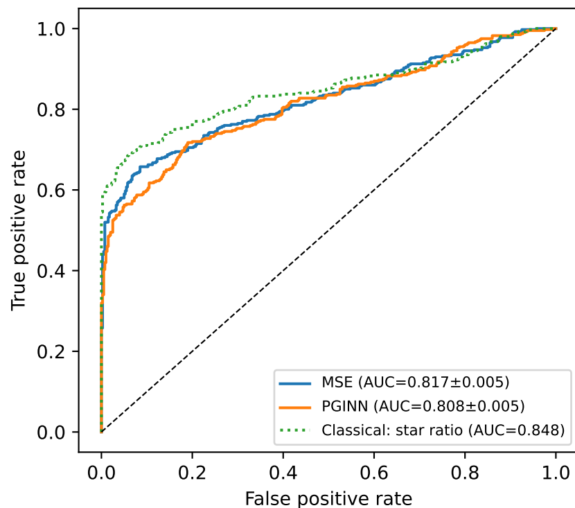
1 locus, n=20
