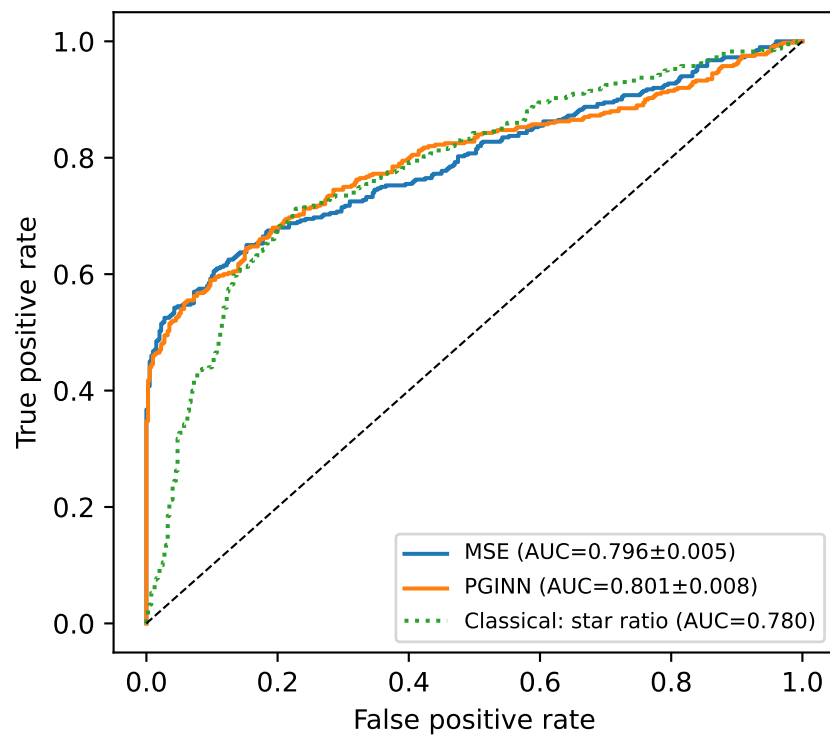
1 locus, n=20
