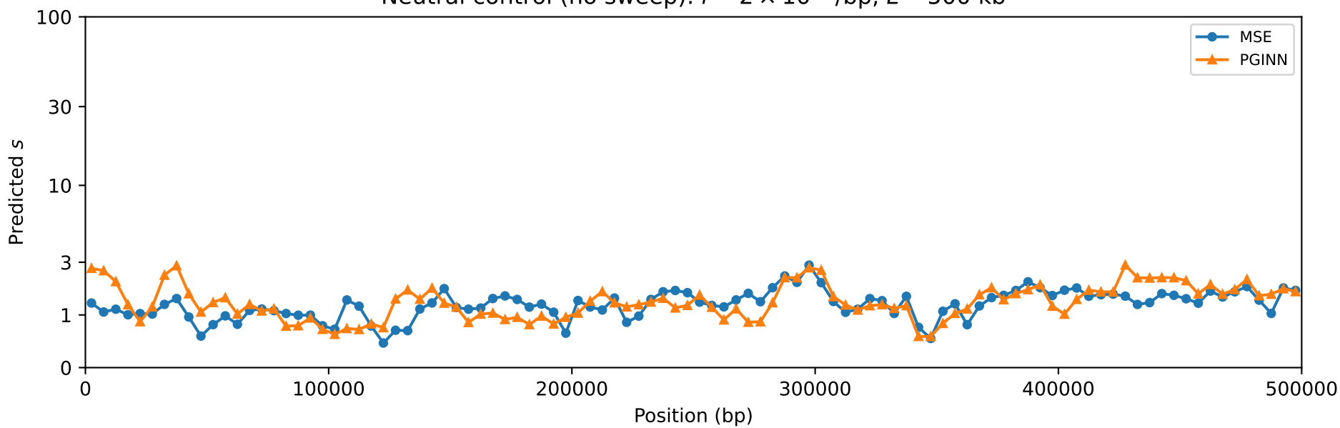
Neutral control (no sweep): r = 2 \times 10^{-8}/\text{bp} , L = 500 \text{ kb}
