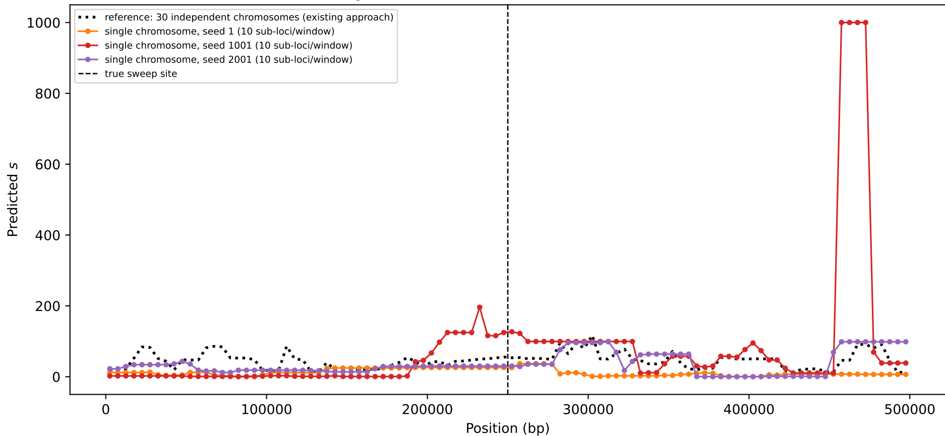
PGINN, r = 2 \times 10^{-8}/\text{bp} , s_g = 0.01 : 100 windows \times 10 sub-loci, single chromosome each
