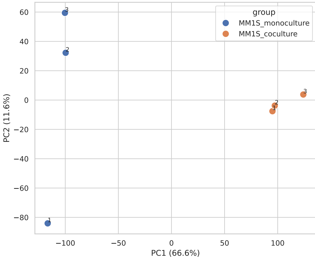
PCA of log2 normalized counts
