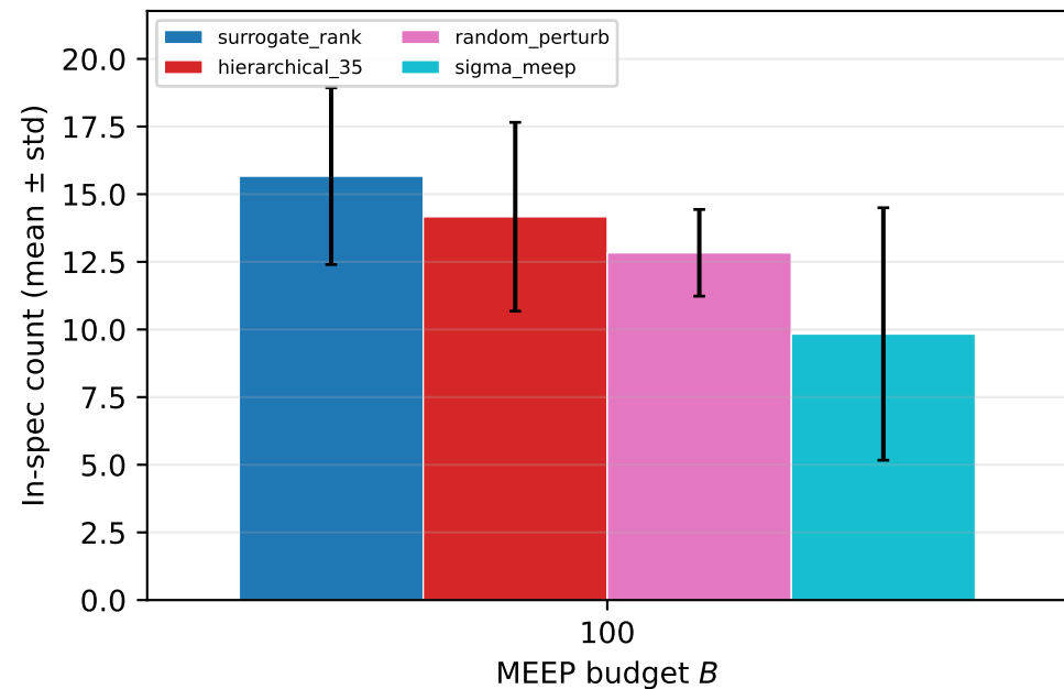
In-spec yield ( n = 6 replicates)
