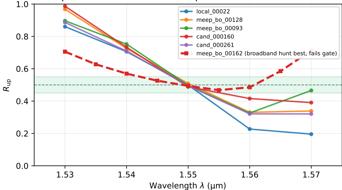
C-band split ratio: narrowband champions vs broadband-aware search
