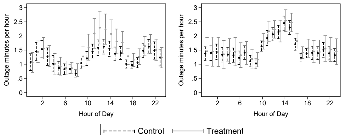
Figure C3: Impacts of transformer injection on outages by time of day A) Before construction B) After construction
