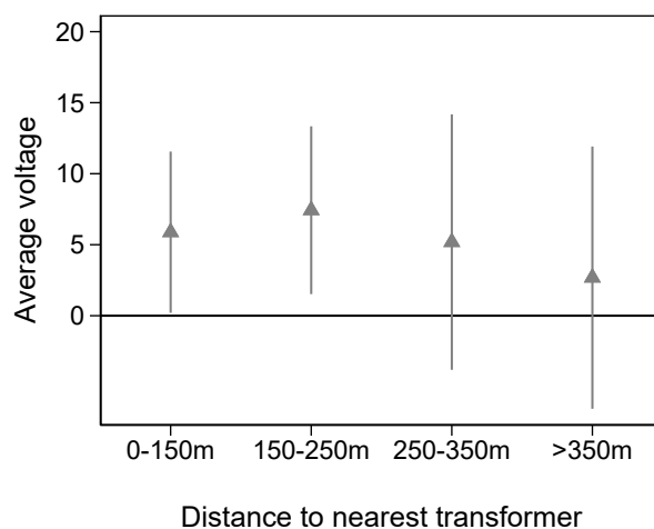
Figure C4: Impact of transformer injection intervention by distance to the nearest transformer at baseline
