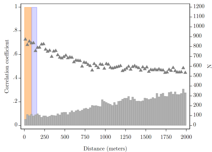
Figure C2: Power quality is highly correlated within short distances
