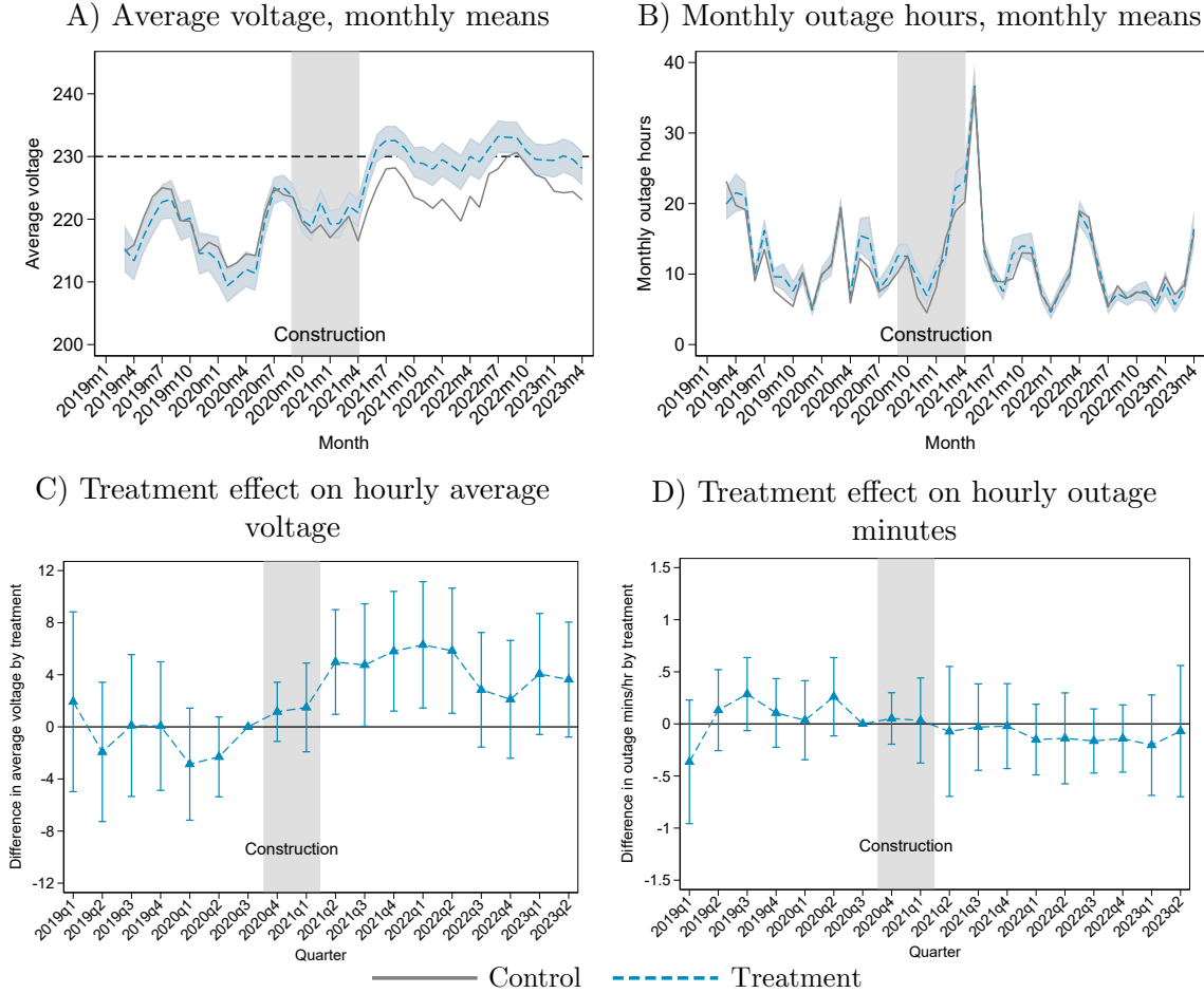
Figure A10: Impacts of transformer injection intervention on power quality and reliability
