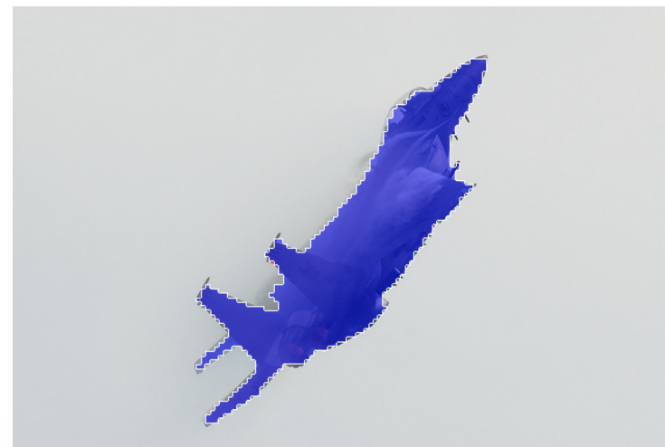
SAM3
