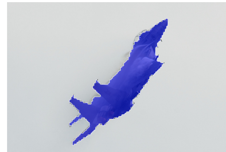
SAM2.1 L
