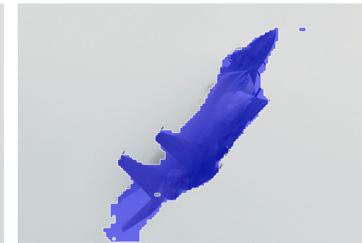
PicoSAM3
