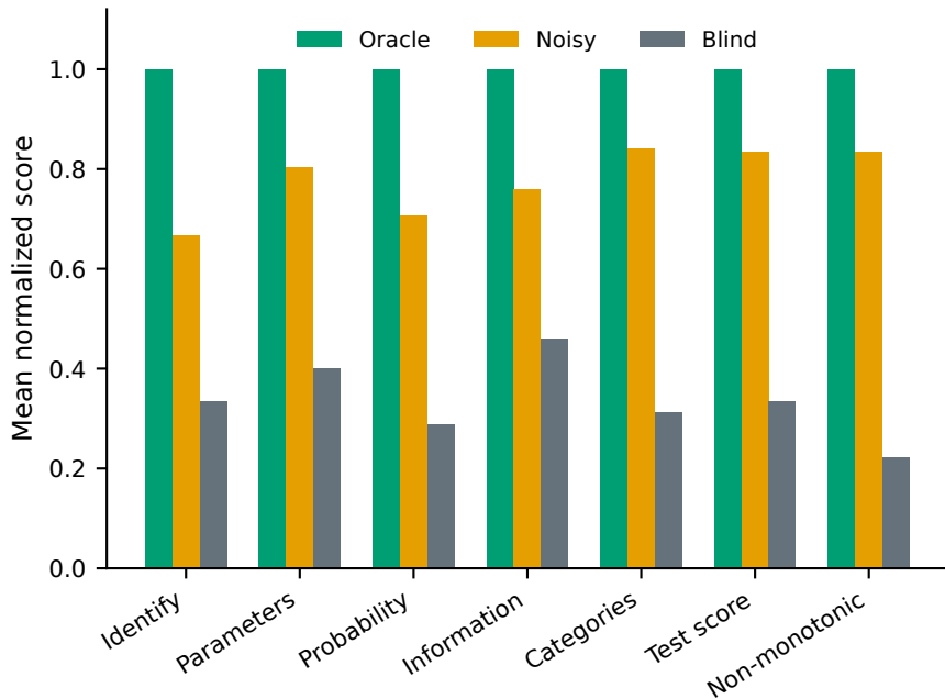
Separation across task families
