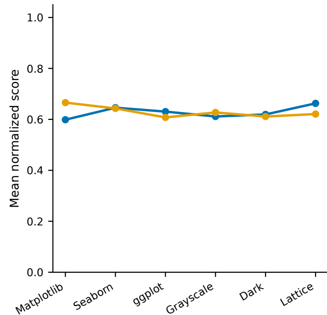
Rendering profile
