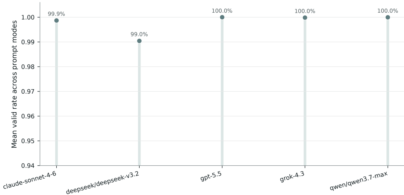
Primary-validity rate by model
