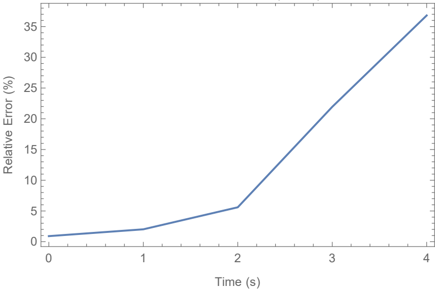
Relative error for F_0=1, G_0=0, a=1
