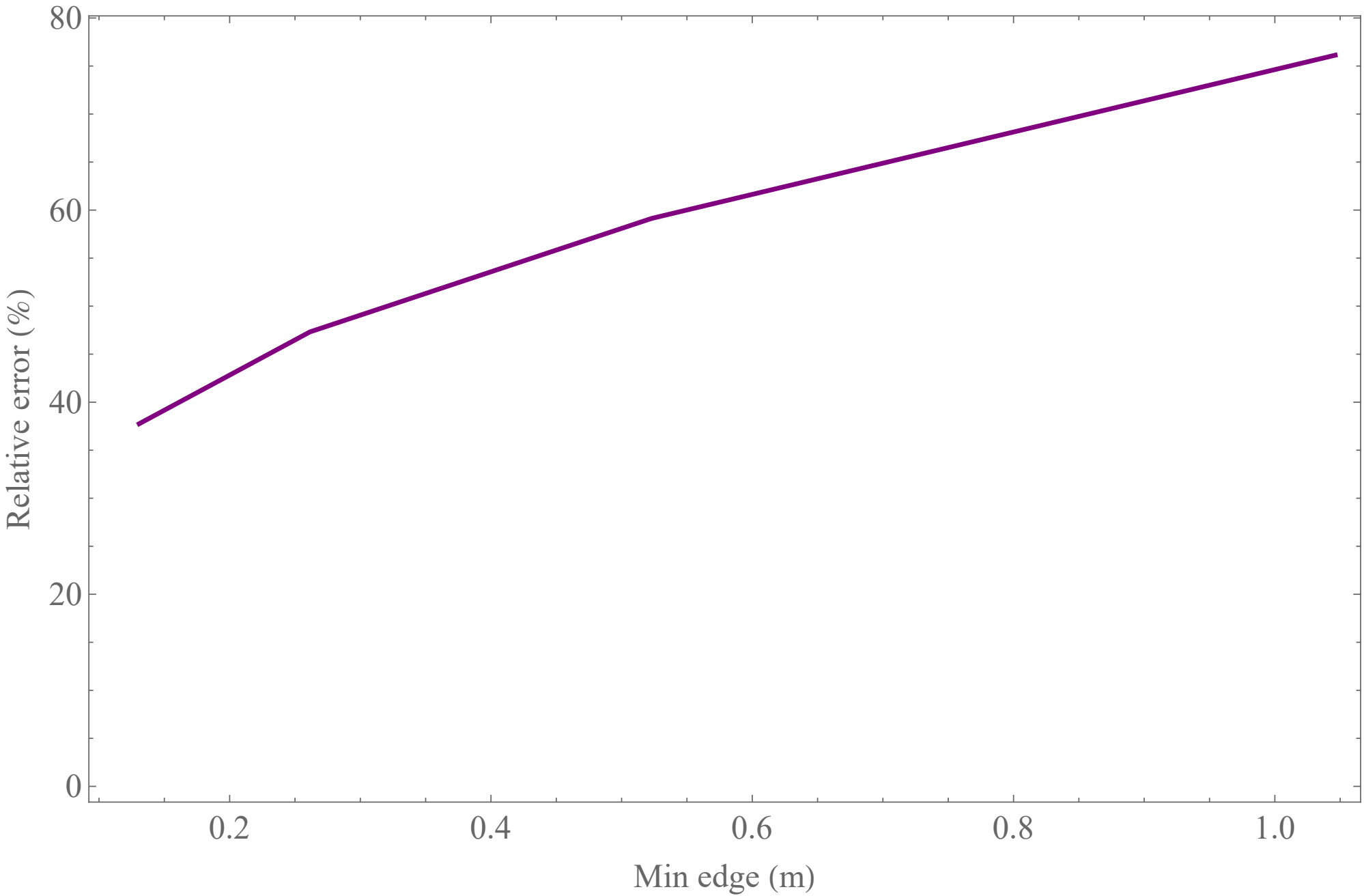
Relative error for F0=1, G0=0, a=1
