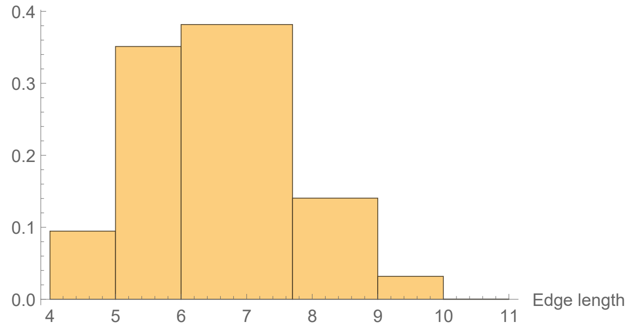
Distribution of mesh edge lengths
