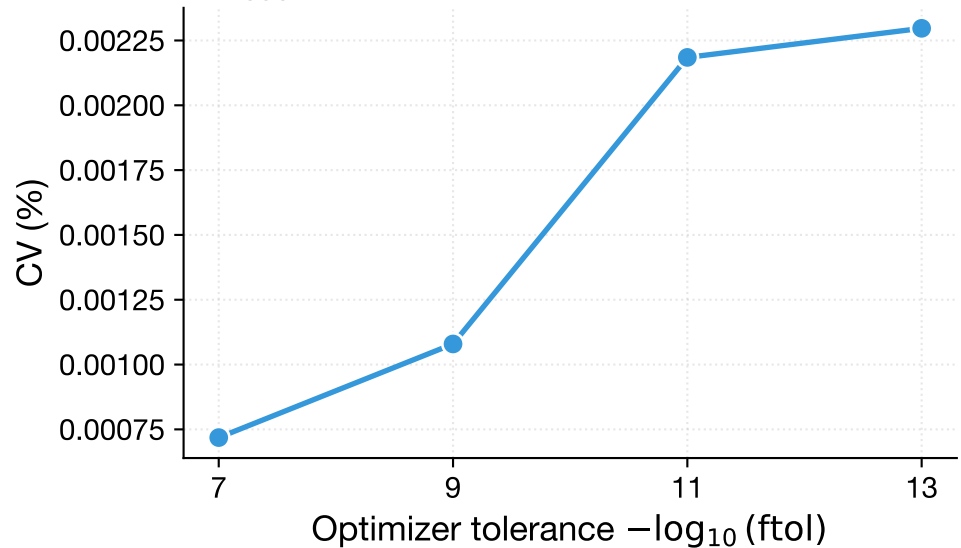
(b) CV of \hat{\mu}
