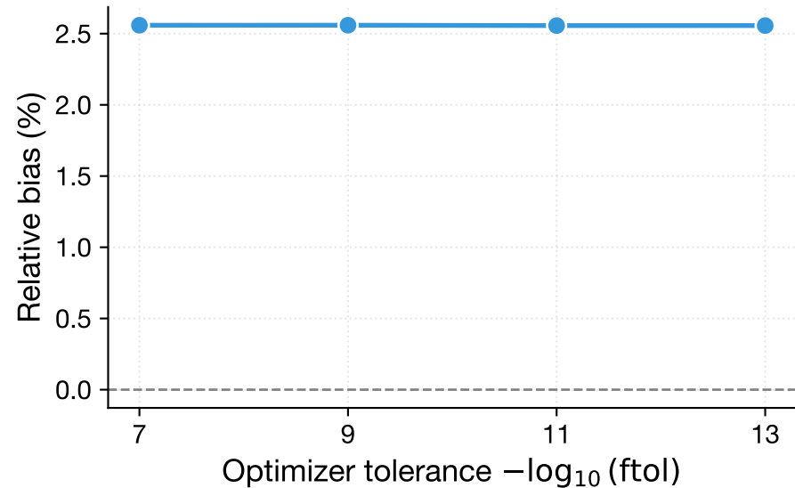
(a) Bias of \hat{\mu}
