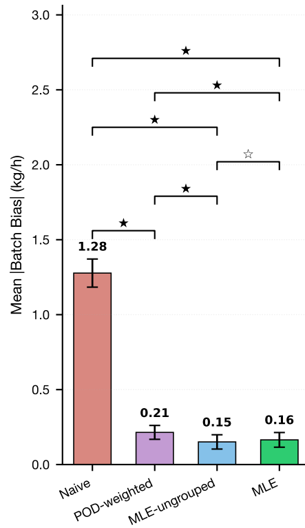
(c) Mean |Batch Bias|
