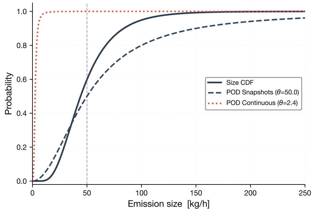
(b) Size CDF and Detection Probability
