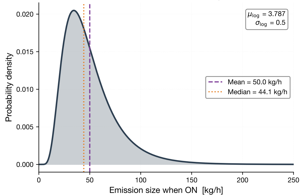
(a) Emission Size Distribution (Lognormal)
