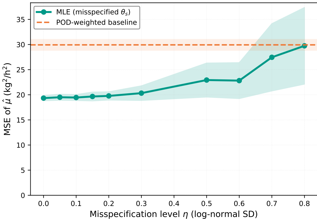
MSE of \hat{\mu}_{\text{MLE}} vs misspecification of \theta_s
