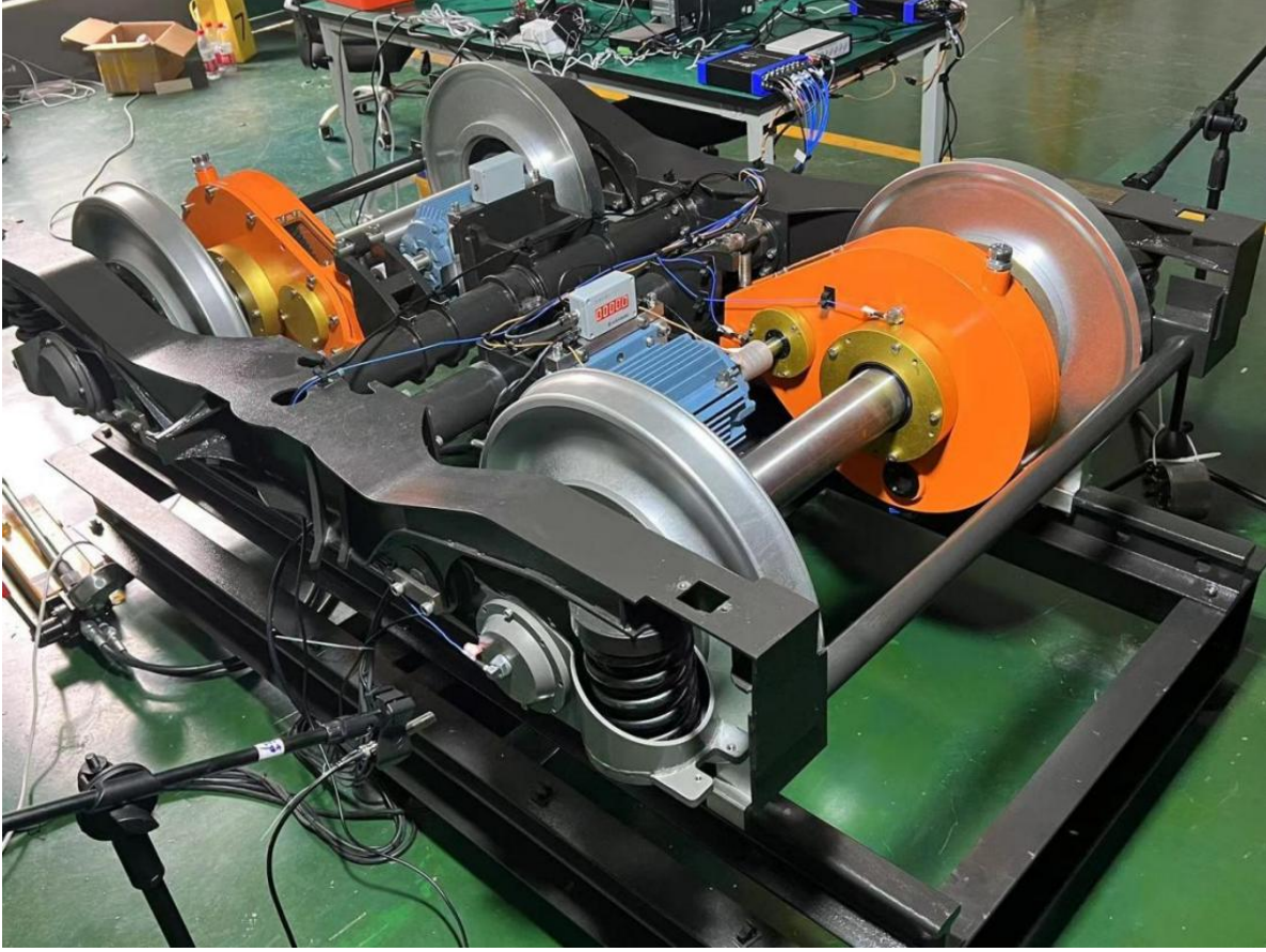
Figure 3: BJTU-RAO dataset experimental platform.
