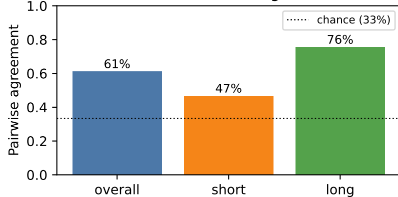
(b) Human-vs-LLM agreement
