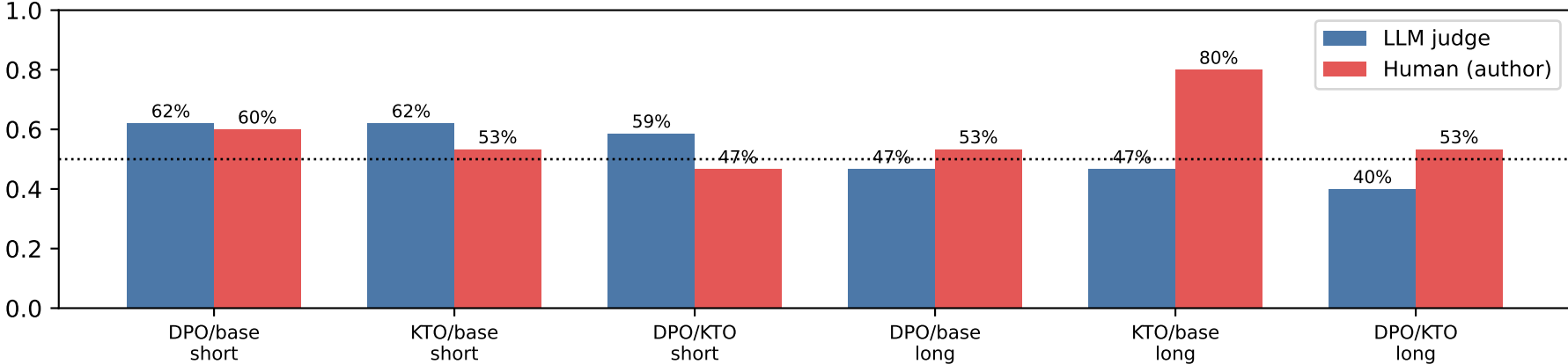
(a) Win rates: LLM vs human
