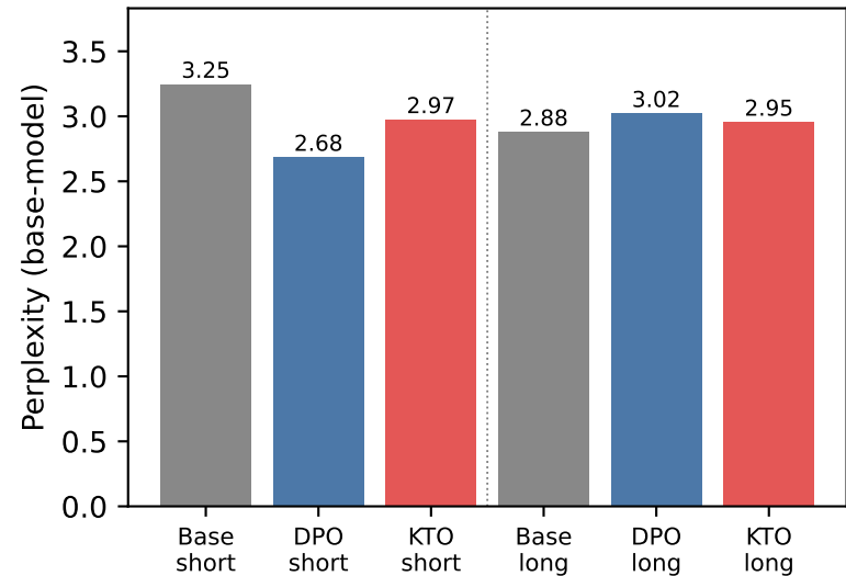
(a) Perplexity
