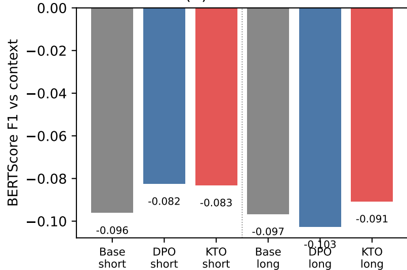
(b) BERTScore
