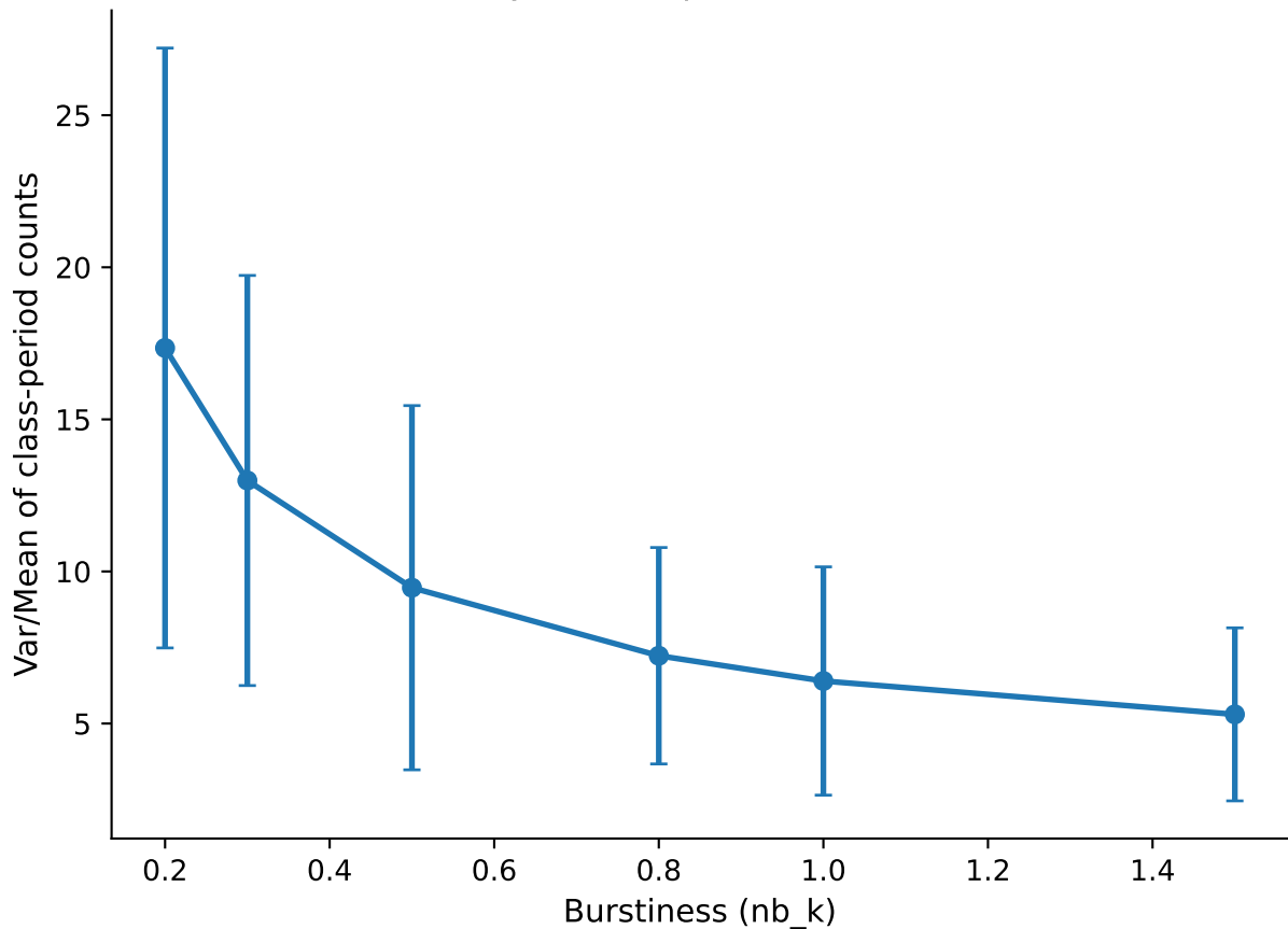
Sensitivity: Overdispersion vs Burstiness
