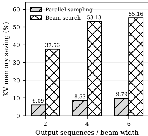
(b) vLLM reported KV-sharing savings
