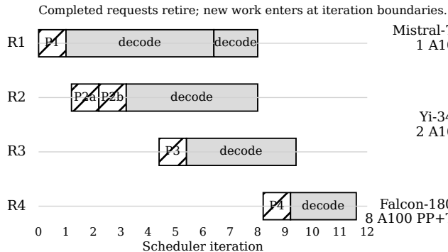
(a) Iteration-level admission with bounded prefill chunks
