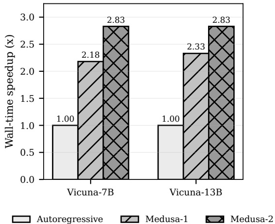
(b) Medusa reported speedups
