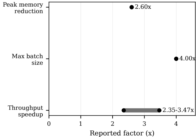
(a) KIVI 2-bit KV-cache results
