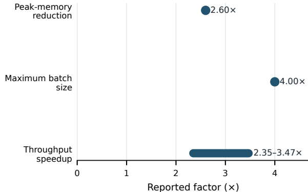
(a) KIVI 2-bit KV-cache results
