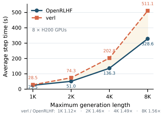
(b) 14B long-CoT RLVR step time
