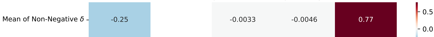
Correlations: Distribution parameters vs Explanatory Variables (S)
