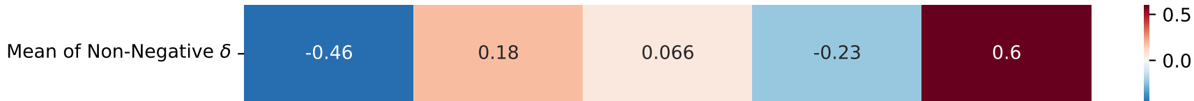
Correlations: Distribution parameters vs Explanatory Variables (E)
