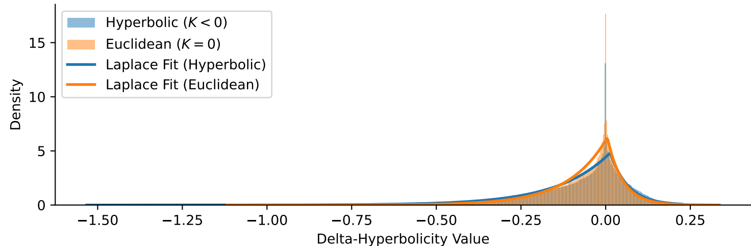
Delta-Hyperbolicity Distributions: Hyperbolic vs Euclidean
