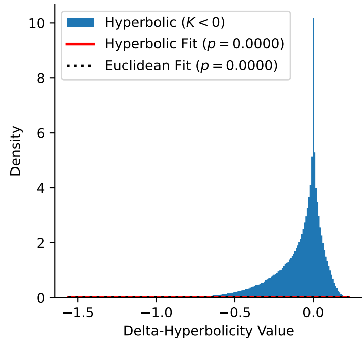
Hyperbolic Data ( K < 0 )
