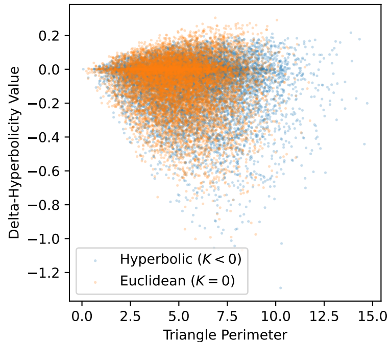
Delta-Hyperbolicity vs Triangle Perimeter
