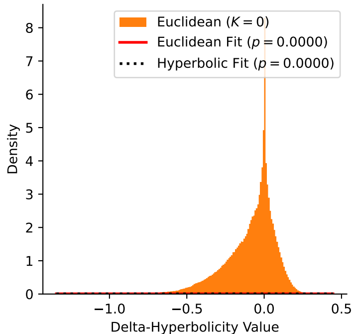
Euclidean Data ( K = 0 )
