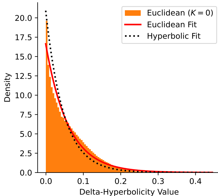
Euclidean Data ( K = 0 )
