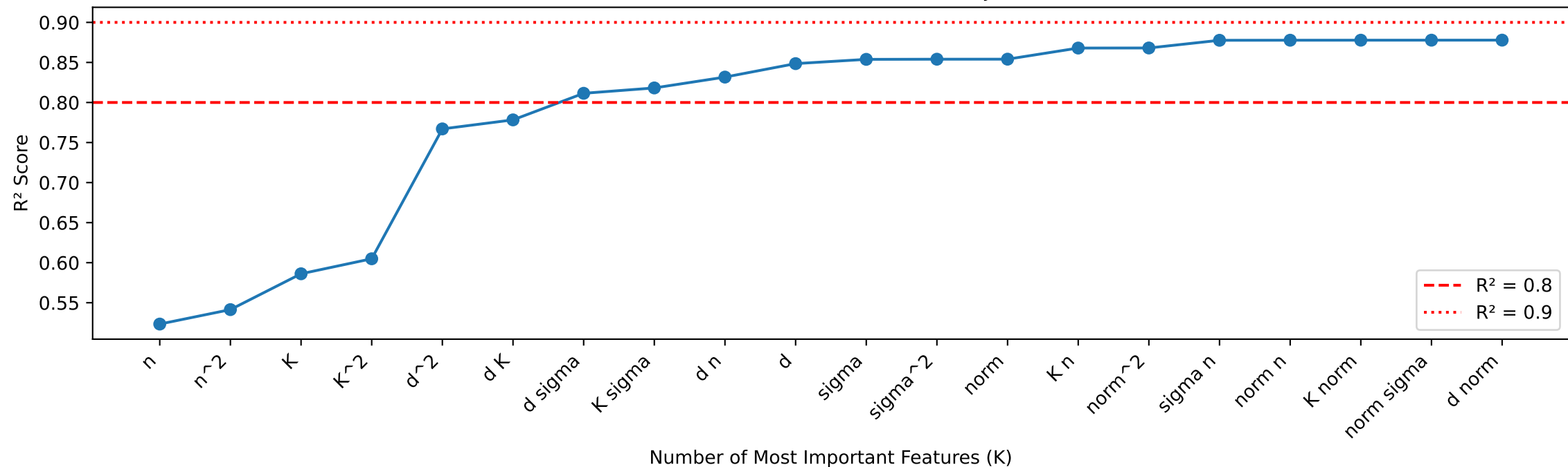
Model Performance vs. Number of Features (Adjusted for Variance)
