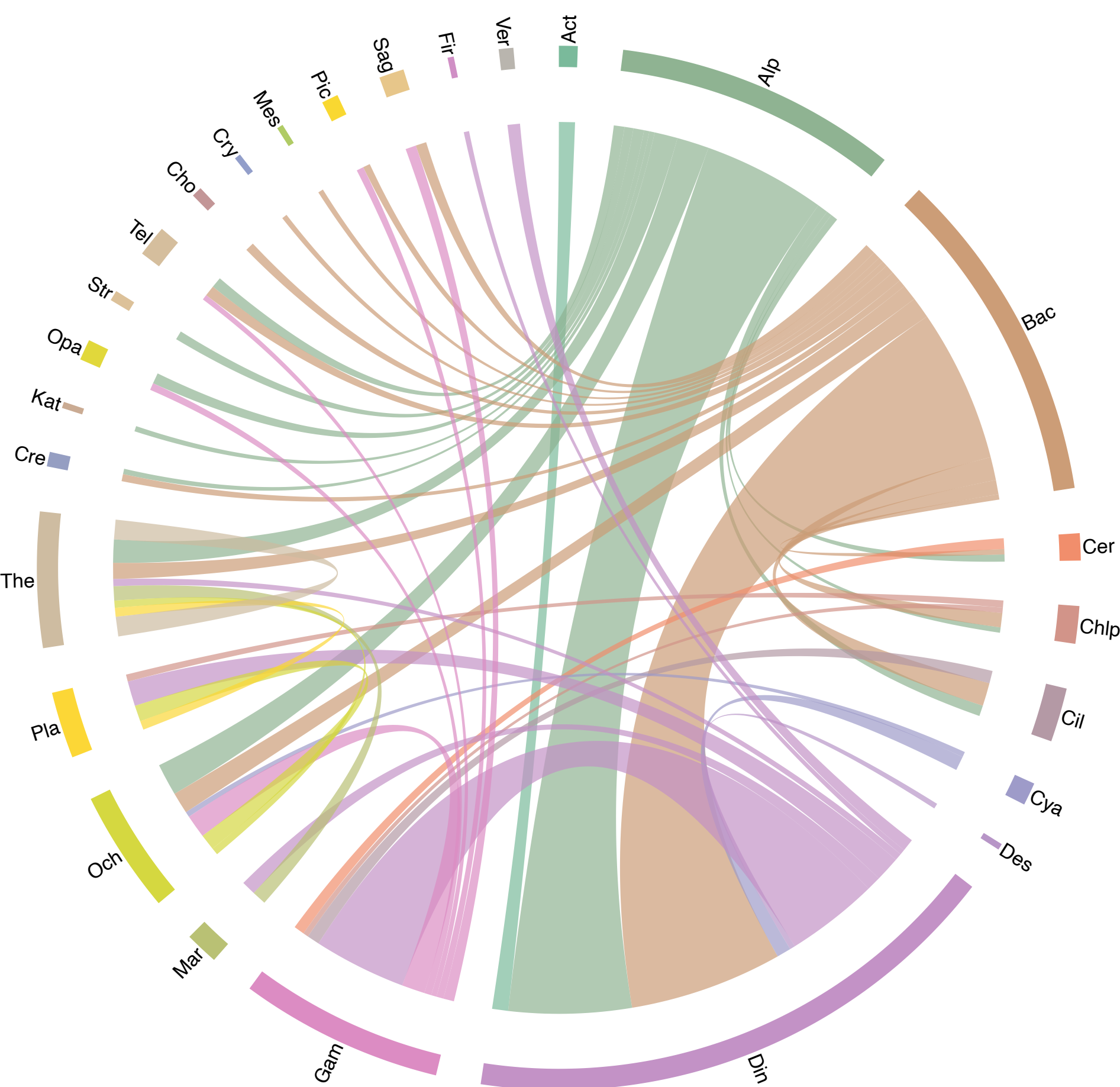
Blanes Bay Microbial Observatory
