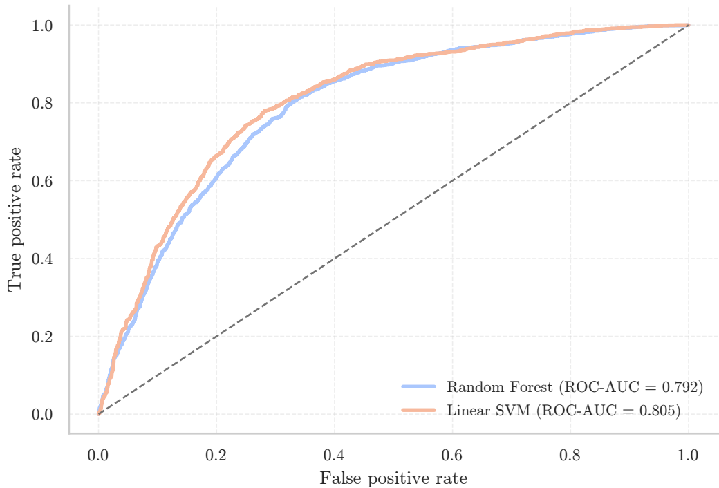
ROC curves
