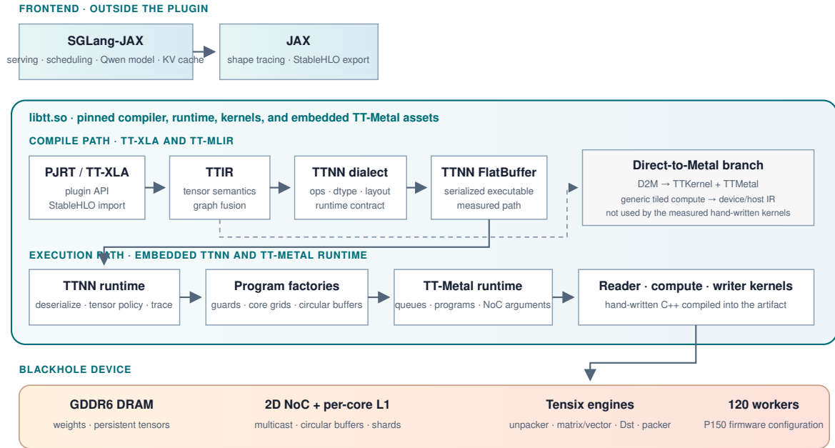
Figure 1: libtt’s serving, compilation, runtime, and device layers.
