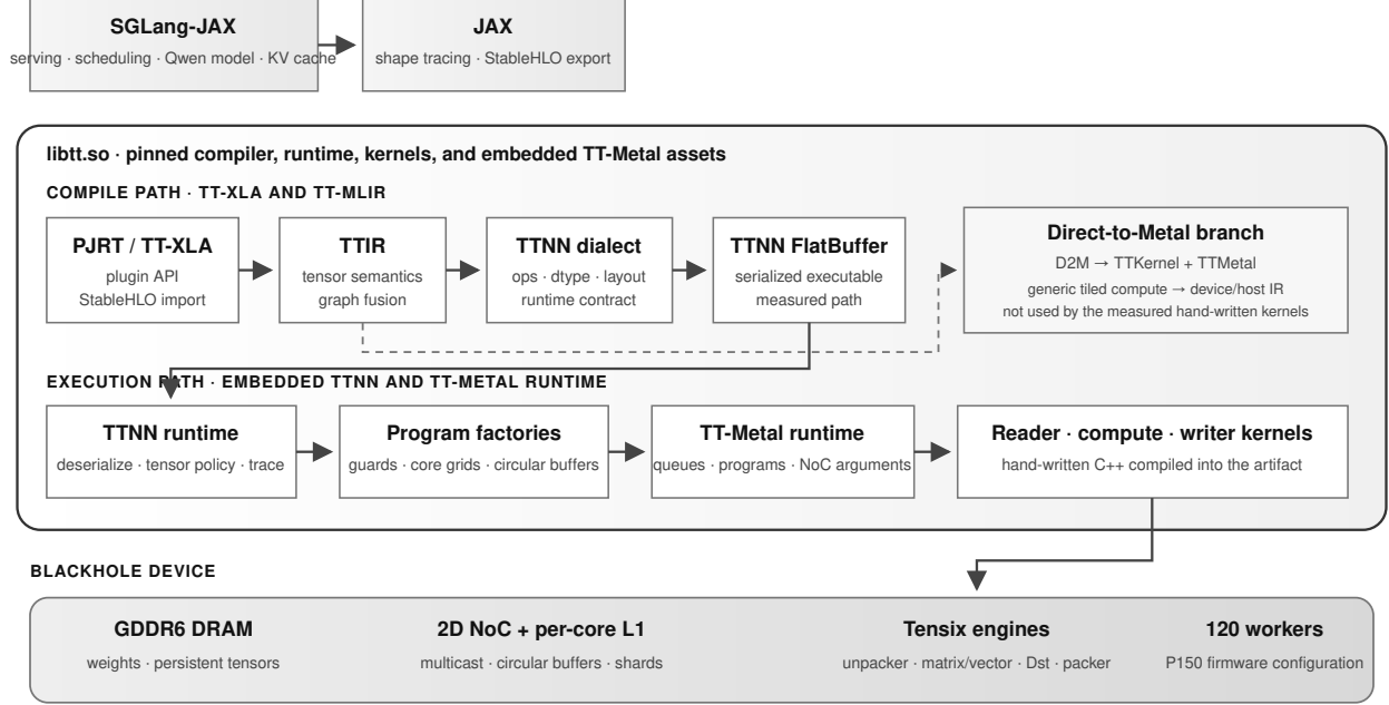
Figure 1: libtt serving, compilation, runtime, and device layers.
