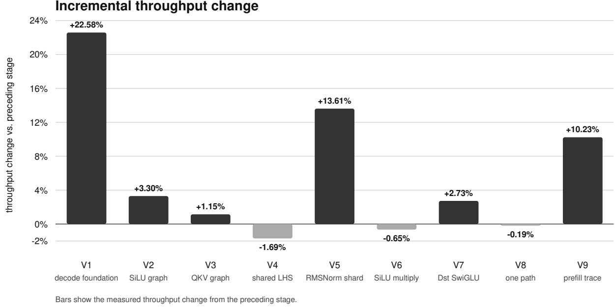
Figure 3: Incremental effect of each concept in the established sequence.
