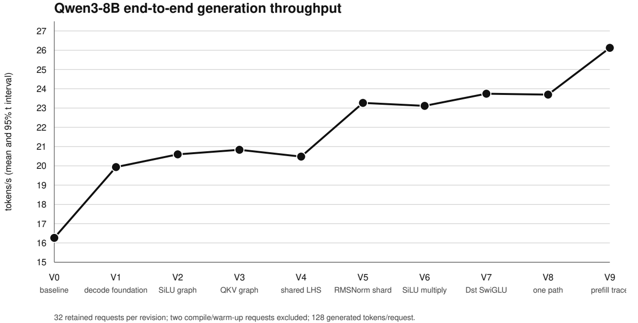
Figure 2: Cumulative throughput across the measured concepts.
