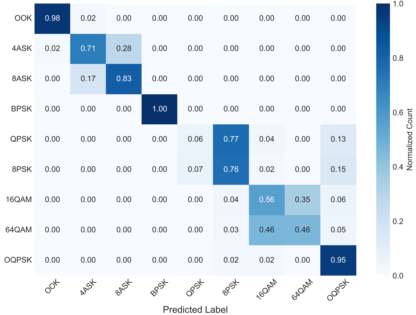
(a) SNR = 0 dB
