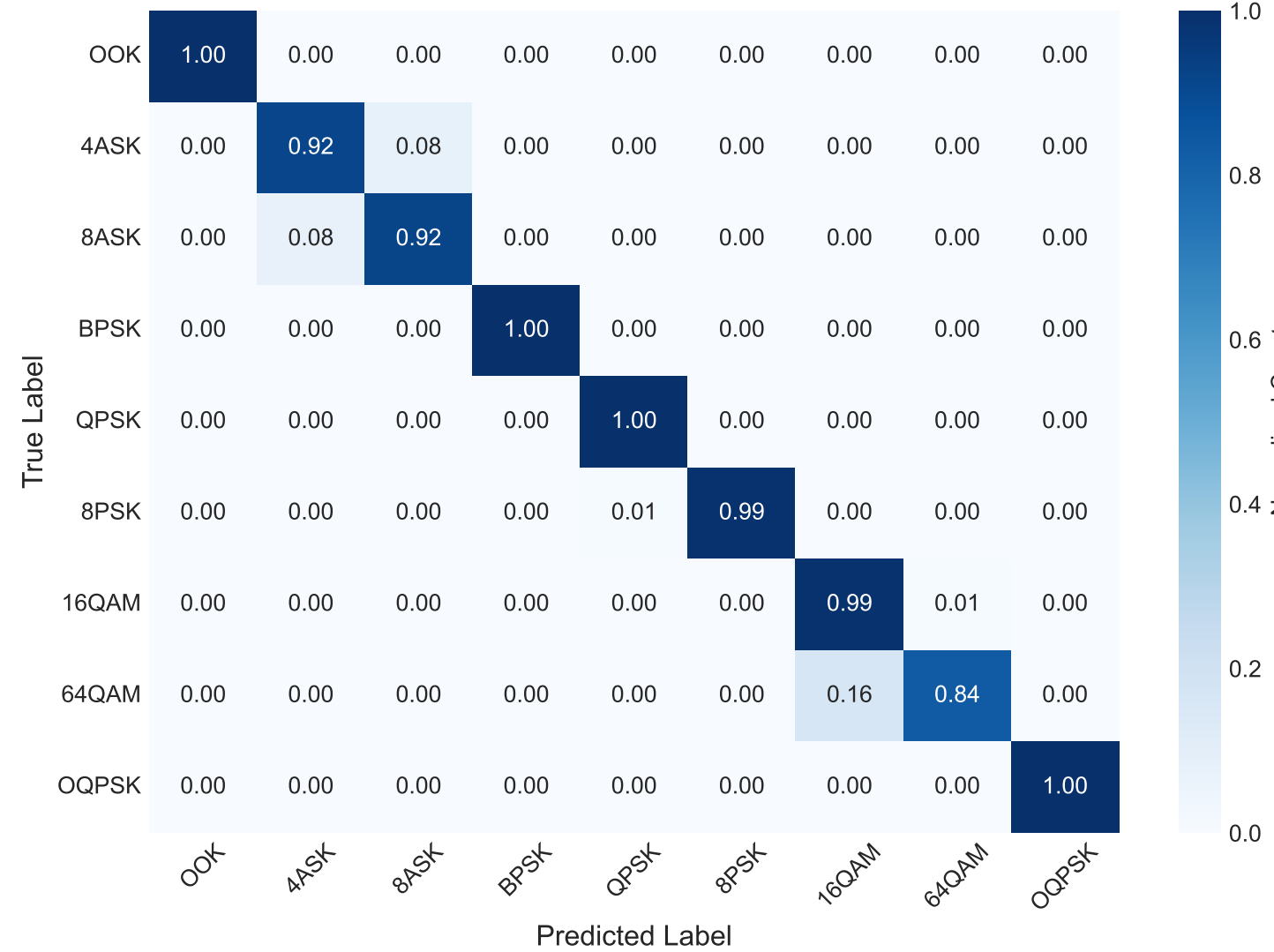
(b) SNR = 8 dB
