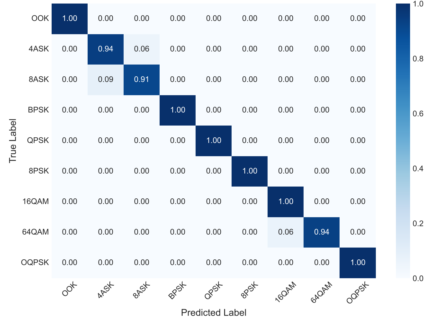
(c) SNR = 30 dB
