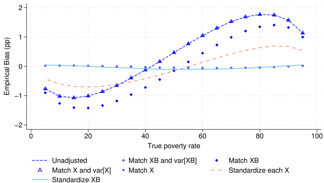
Figure 10: Bias in FGT0 under top and bottom biased samples (Sec 4.4.1) and different correction measures
