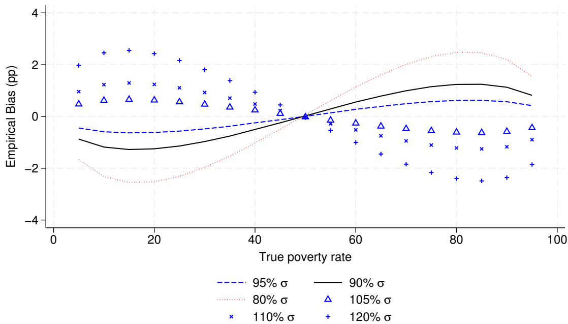
Figure 13: Change in poverty prediction if \sigma changes by x\%
