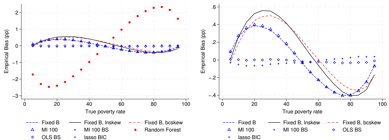
Figure 3: Bias in FGT0 of different methods under non-normal errors
