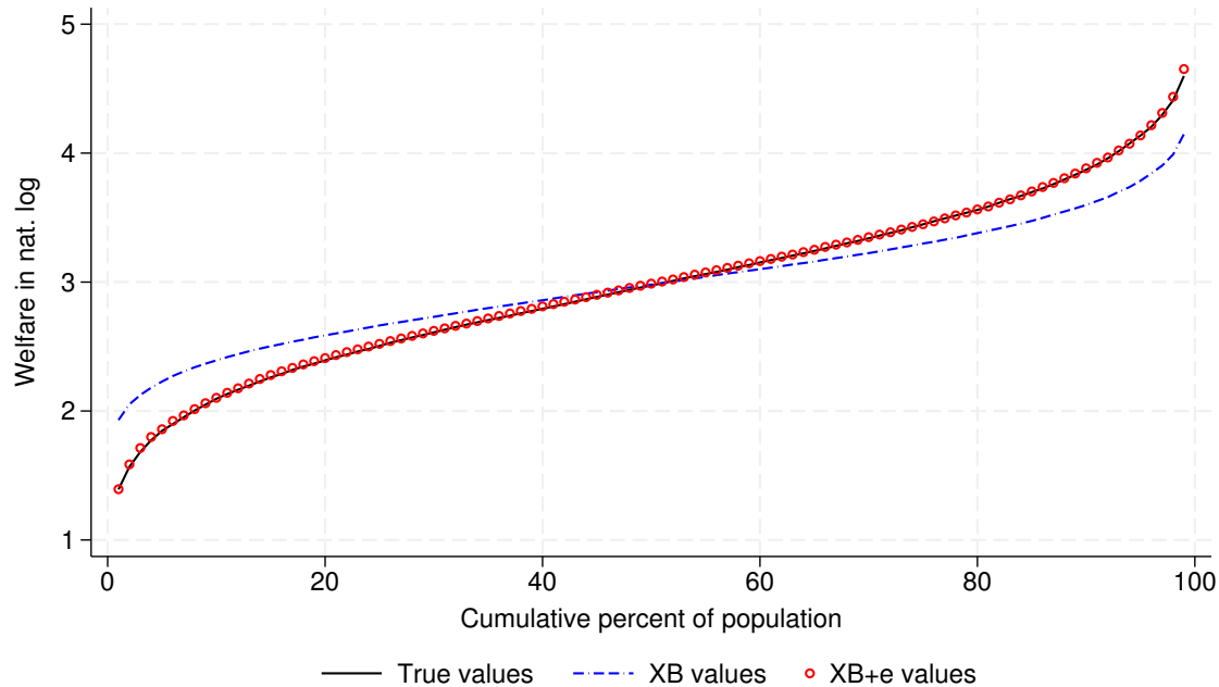
Figure 1: Replicating the actual distribution, with and without simulated errors
