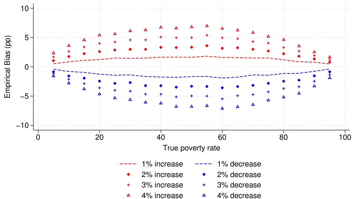
Figure 14: Resulting poverty prediction if constant term changes by x\%
