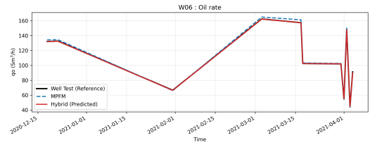
(b) W06 oil rate temporal generalization performance
