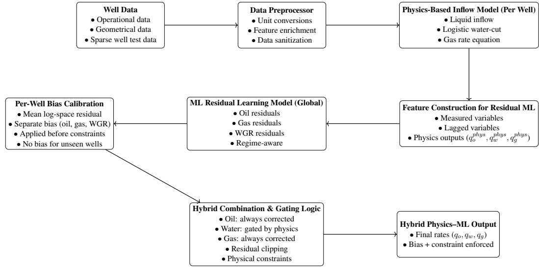
Figure 3.1 Hybrid physics-informed residual learning architecture for virtual flow metering
