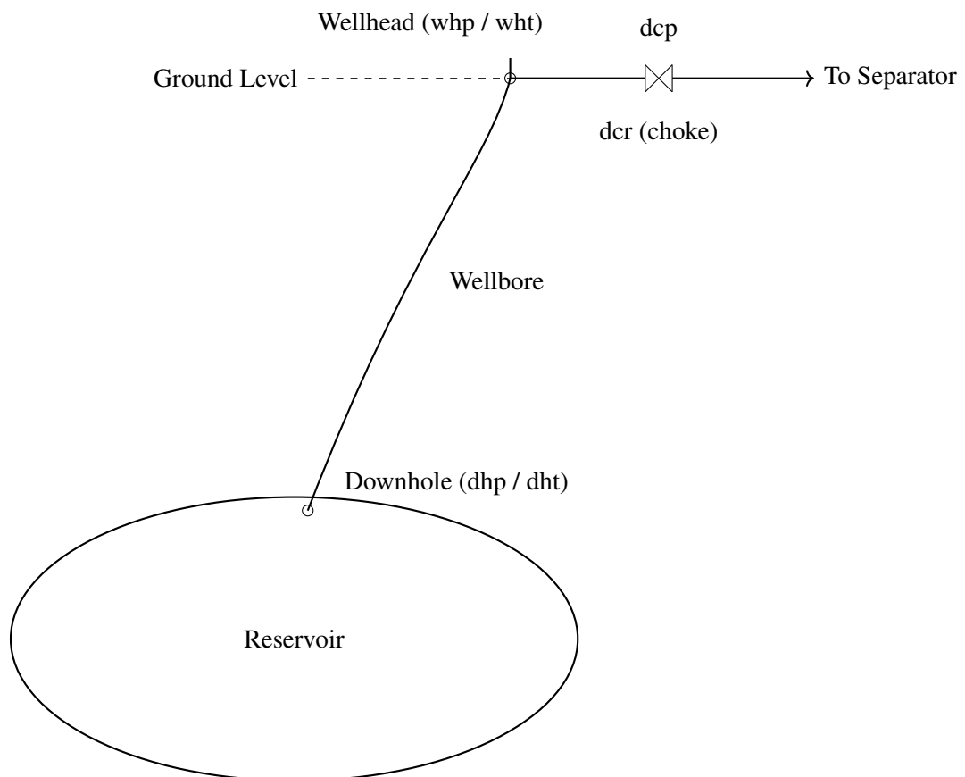
Figure 1.2 Well instrumentation setup
