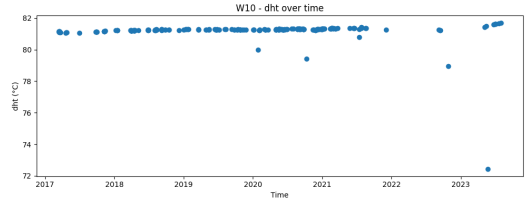
Figure 3.3 W10 – Downhole temperature
