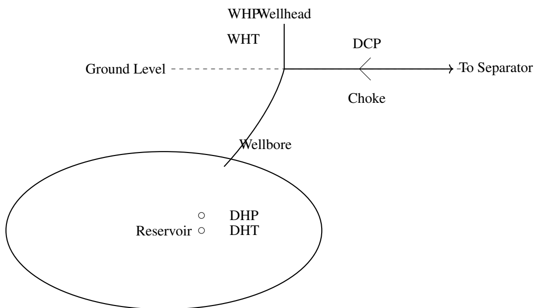
Figure 1.2 Well Flow Measurement Instrumentation Setup
