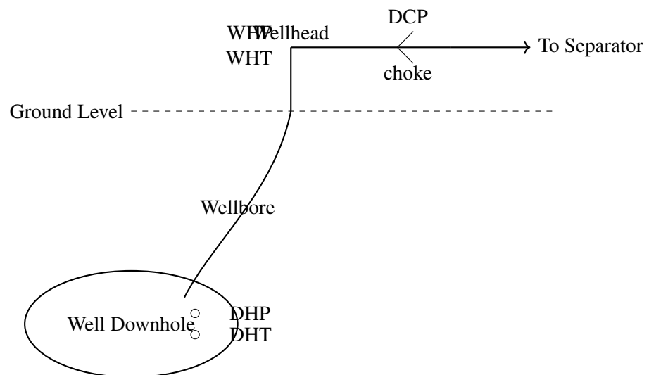
Figure 1.2 Well Downhole and Surface Instrumentation
