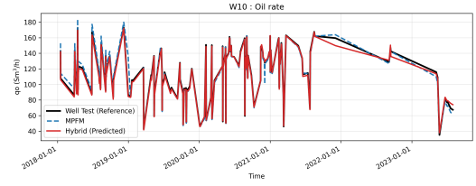
(b) W10 oil rate spatial generalization performance
