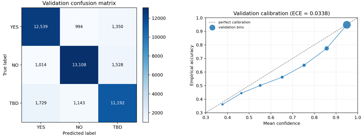
Figure 4: Evaluation artifacts derived from the S12B certification record. Left: validation confusion matrix. Right: validation calibration curve with ECE = 0.0338.
