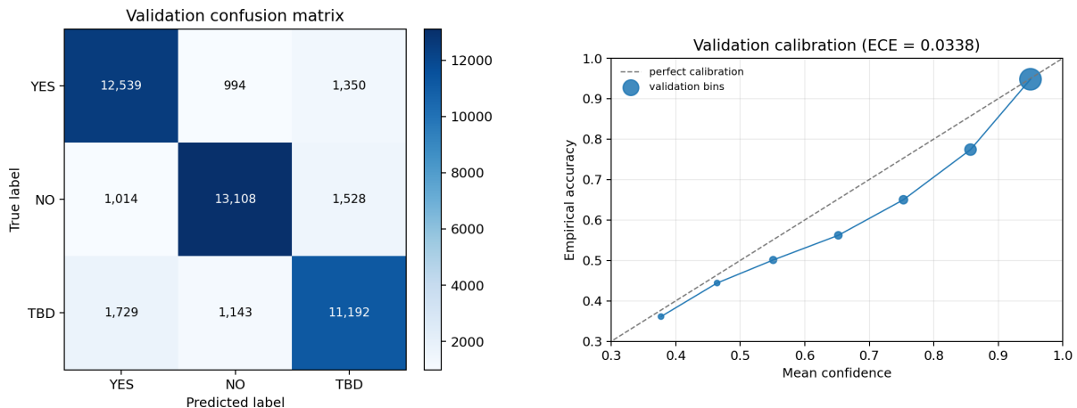
Figure 4: Evaluation artifacts derived from the S12B certification record. Left: validation confusion matrix. Right: validation calibration curve with ECE = 0.0338 .
