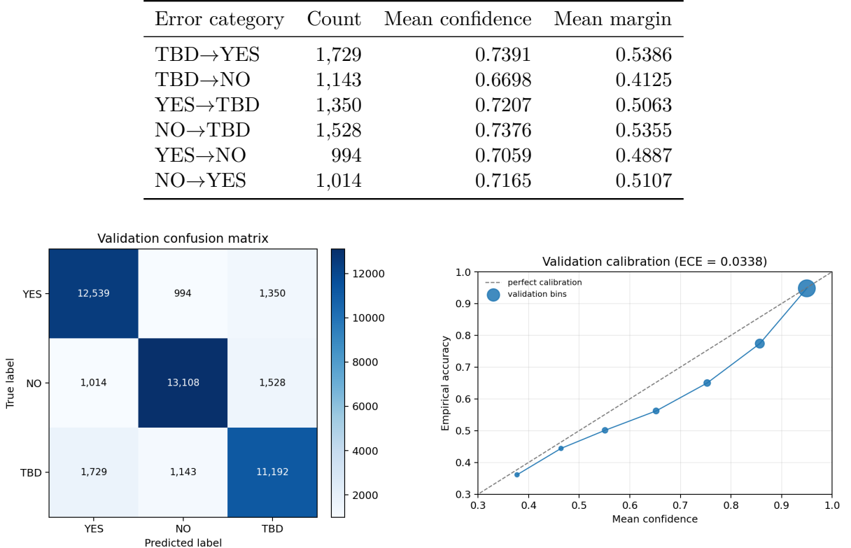
Figure 4: Evaluation artifacts derived from the S12B certification record. Left: validation confusion matrix. Right: validation calibration curve with ECE = 0.0338 .
