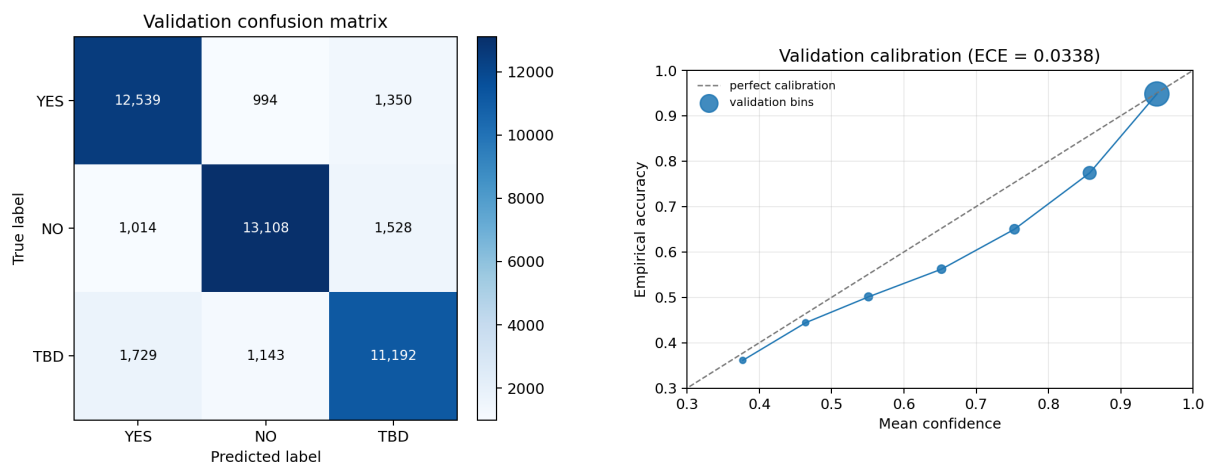
Figure 2: Evaluation artifacts derived from the S12B certification record. Left: validation confusion matrix. Right: validation calibration curve with ECE = 0.0338 .
