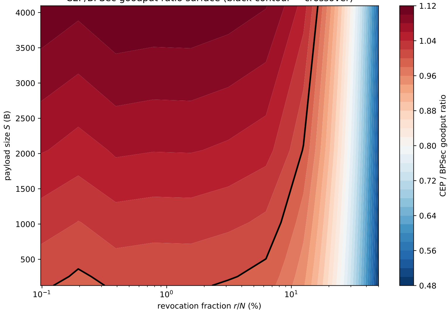
CEP/BPsec goodput ratio surface (black contour = crossover)
